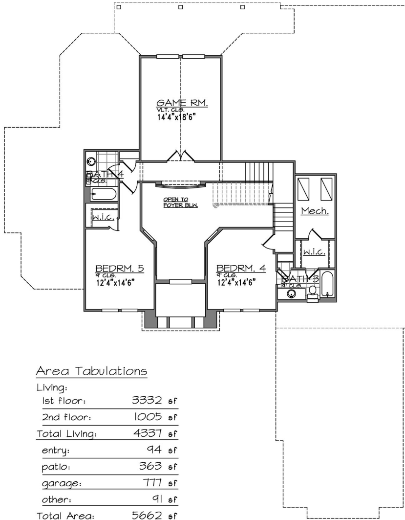
2nd. Floor Plan
